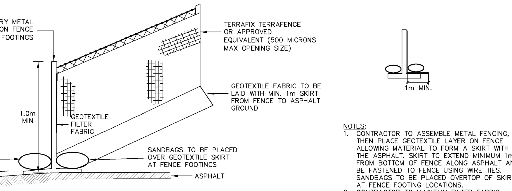
SEDIMENT CONTROL FILTER FABRIC FENCE ON ASPHALT N.T.S.
